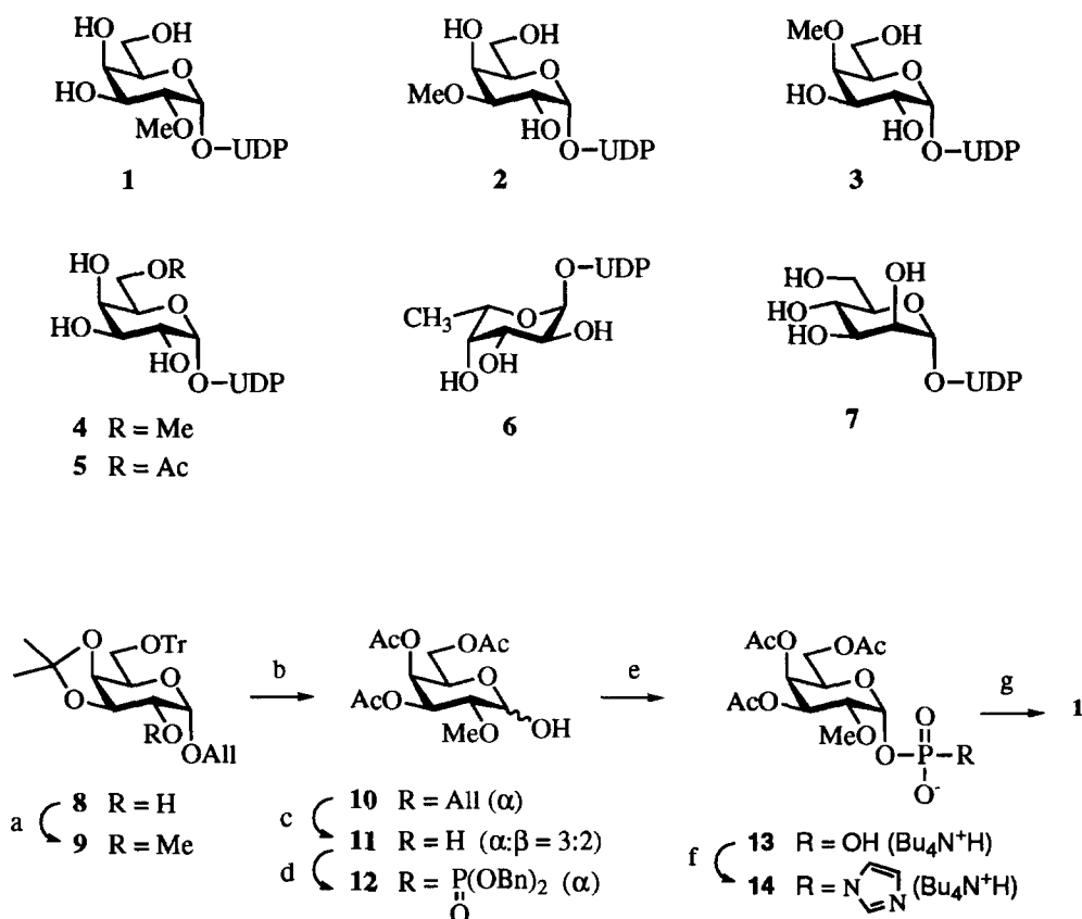
Scheme 1. (a) MeI, NaH/DMF, 97%; (b) (1) 70% AcOH, 60 °C, (2) Ac 2 O/pyridine, 93.5% (2 steps); (c) (1) Pd-C/MeOH, 60 °C, (2) HgCl 2 , HgO/acetone-H 2 O, 79% (2 steps); (d) BuLi, (BnO) 2 POCl/THF, -78 °C \alpha -anomer 34%, \beta -anomer 10%; (e) H 2 , Pd-C, Bu 3 N/MeOH; (f) N,N' -carbonyldimidazole/DMF; (g) (1) UMP·Bu 3 N/DMF, (2) Et 3 N-MeOH-H 2 O, 14% from 12 .
