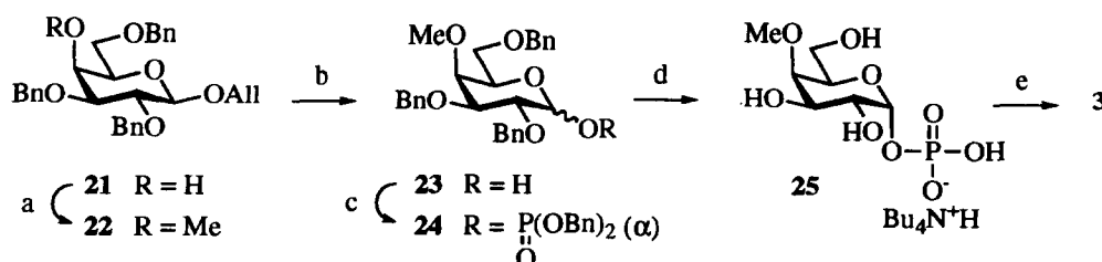
Scheme 3. (a) \text{MeI} , \text{NaH}/\text{DMF} , 73.5%; (b) (1) t\text{-BuOK}/\text{DMSO} , 60^\circ\text{C} , (2) \text{HgCl}_2 , \text{HgO}/\text{acetone-H}_2\text{O} , quant. (2 steps); (c) \text{BuLi} , (\text{BnO})_2\text{POCl}/\text{THF} , -78^\circ\text{C} 45%; (d) \text{H}_2 , \text{Pd-C} , \text{Bu}_3\text{N}/\text{MeOH} ; (e) \text{UMP-imidazole}/\text{DMF} , 11% from 24 .
