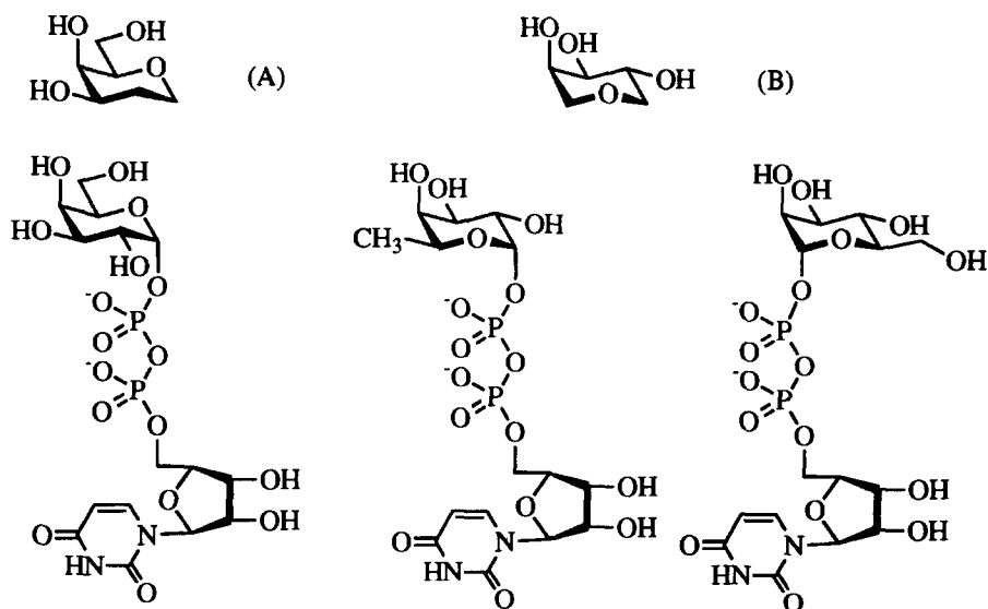
Figure 1. Alternative structure unit (B) of UDP-Fuc and UDP-Man effective for the binding as well as that (A) of UDP-Gal.
