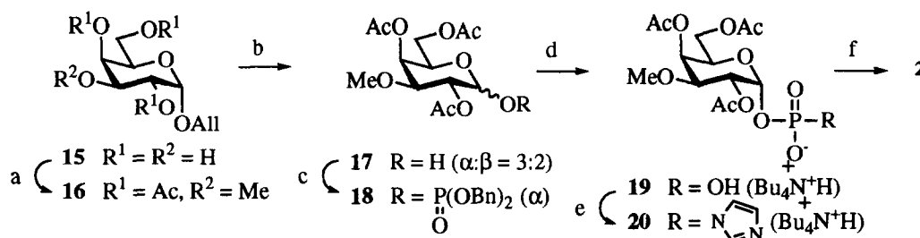
Scheme 2. (a) (1) \text{Bu}_3\text{SnO}/\text{MeOH} , reflux, (2) \text{MeI} , \text{Bu}_3\text{NI}/\text{toluene} , reflux, (3) \text{Ac}_2\text{O}/\text{pyridine} , 71% (3 steps); (b) (1) \text{Pd-C}/\text{MeOH} , 60^\circ\text{C} , 2) \text{HgCl}_2 , \text{HgO}/\text{acetone-H}_2\text{O} , 64%; (c) \text{BuLi} , (\text{BnO})_2\text{POCl}/\text{THF} , -78^\circ\text{C} , 41%; (d) \text{H}_2 , \text{Pd-C} , \text{Bu}_3\text{N}/\text{MeOH} ; (e) N,N' -carbonyldimidazole/ \text{DMF} ; (f) (1) \text{UMP}\cdot\text{Bu}_3\text{N}/\text{DMF} , (2) \text{Et}_3\text{N-MeOH-H}_2\text{O} , 10% from 18 .
