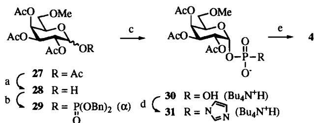
Scheme 4. (a) \text{H}_2\text{NNH}_2 , AcOH, 60 °C; (b) BuLi, (\text{BnO})_2\text{POCl/THF} , -78 °C 49%; (c) \text{H}_2 , Pd-C, \text{Bu}_3\text{N/Me} ; (d) N,N' -carbonyldimidazole/DMF; (e) 1) \text{UMP}\cdot\text{Bu}_3\text{N/DMF} , 2) \text{Et}_3\text{N-MeOH-H}_2\text{O} , 22% from 29 .
