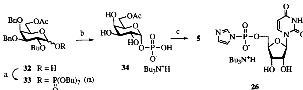
Scheme 5. (a) t\text{-BuLi} , (\text{BnO})_2\text{POCl/THF} , -78 °C 35%; (b) \text{H}_2 , Pd-C, \text{Bu}_3\text{N/MeOH} ; (c) \text{UMP-imidazolidine (26)/DMF} , 14% from 24 .
